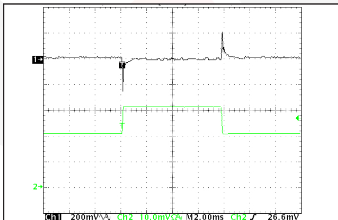
Figure 11: Output voltage response to step-change in load current (50%-75%-50% of I_{out(max)} ); ( dI/dt = 0.1 A/\mu s ). Load cap: 1 µF ceramic and 15 µF tantalum capacitors. Ch 1: V_{out} (200mV/div), Ch 2: I_{out} (10A/div), (2ms/div).
