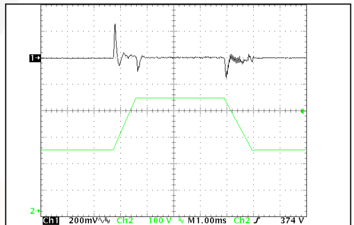
Figure 12: Output voltage response to step-change in input voltage (250V/ms). Load cap: 1µF ceramic and 15µF tantalum capacitors. Ch 1: V_{out} (200mV/div), Ch 2: V_{in} (100V/div), (1ms/div).
