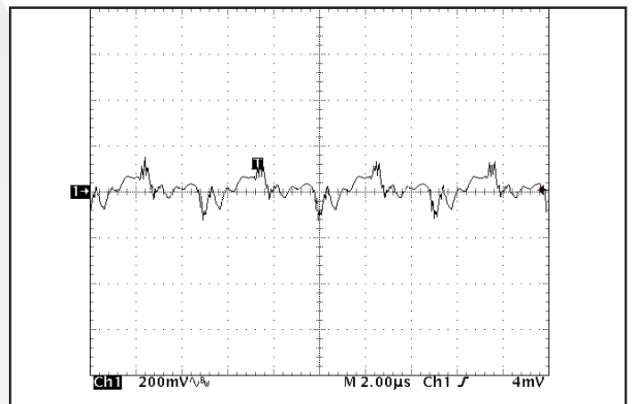
Figure 10: Output voltage ripple, V_{out} , at nominal input voltage and rated load current (200 mV/div), (2µs/div). Load capacitance: 1µF ceramic capacitor and 15µF tantalum capacitor. Bandwidth: 10 MHz. See Figure 17.
